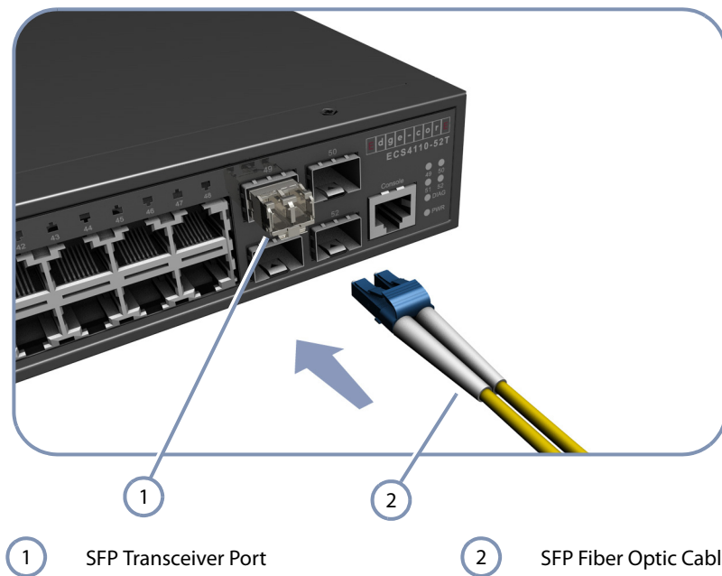
Figure 19: Making a Connection to a SFP Port
