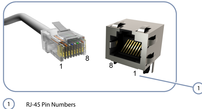
Figure 17: RJ-45 Connector
