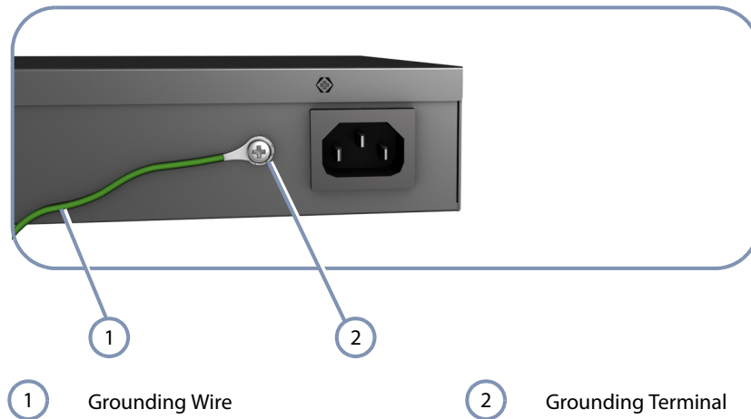
Figure 13: Grounding Terminal
