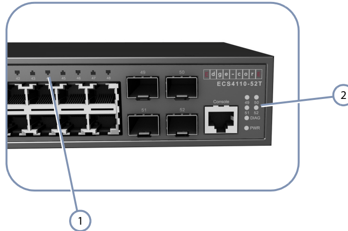
Figure 15: Port Status LEDs
