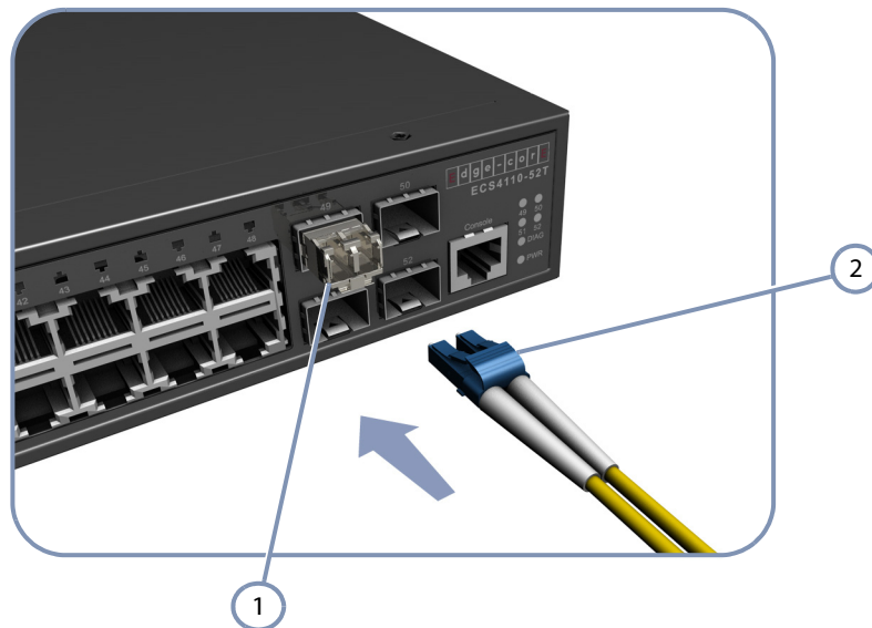
Figure 7: Making a Connection to a SFP Port
