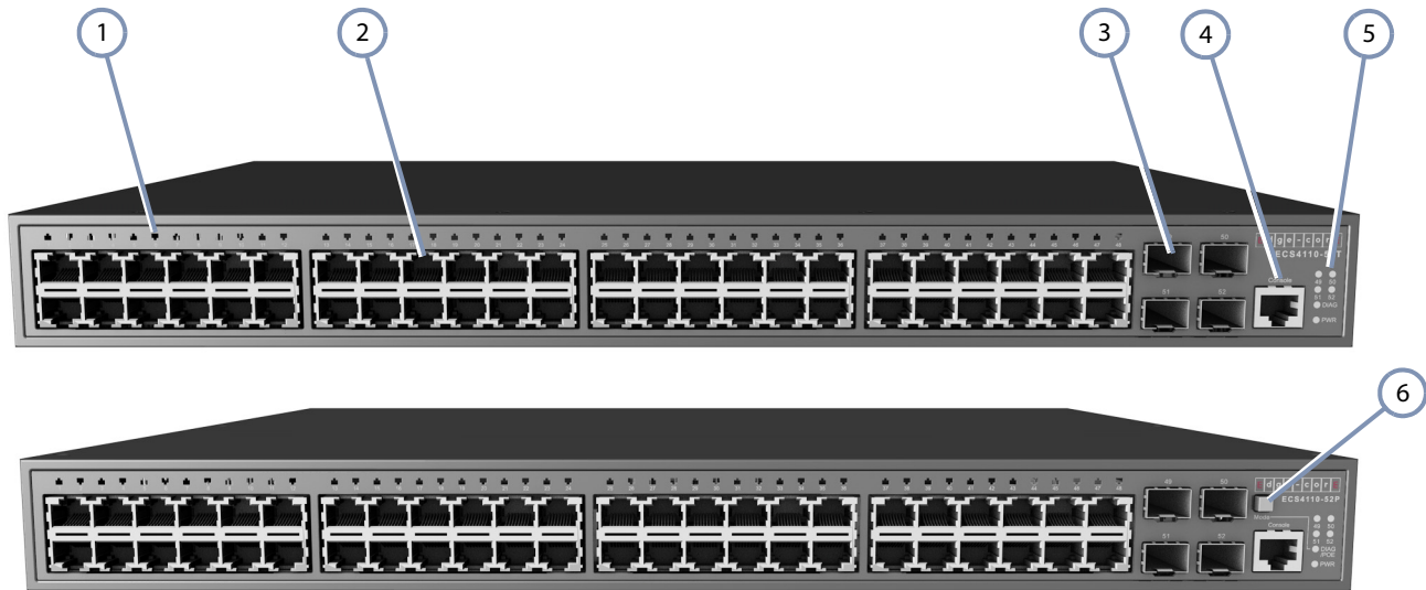
Figure 1: Front Panel ECS4110-52T (upper) and ECS4110-52P (lower)
